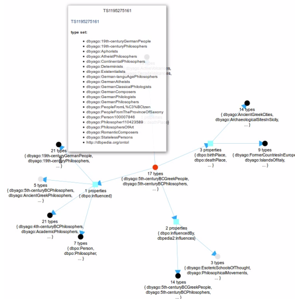
Figure 1. Visualisation of an initial query over induced schema-level patterns in ELLIS.
