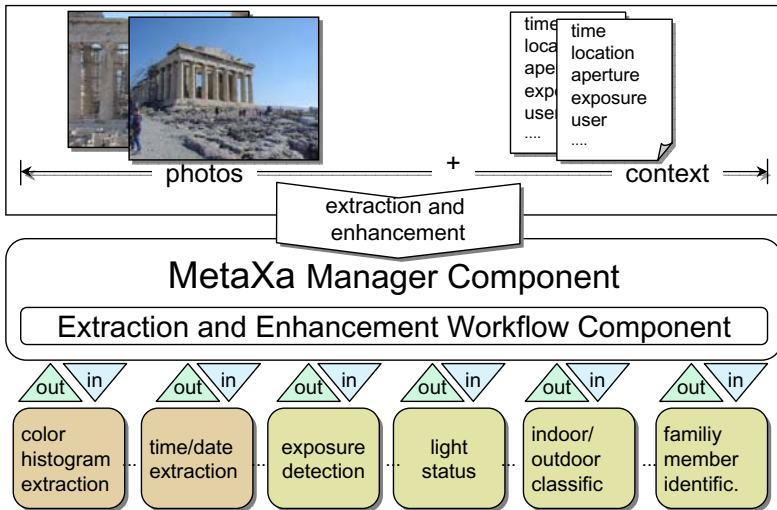
Fig. 1. Metadata extraction and enhancement architecture MetaXa
